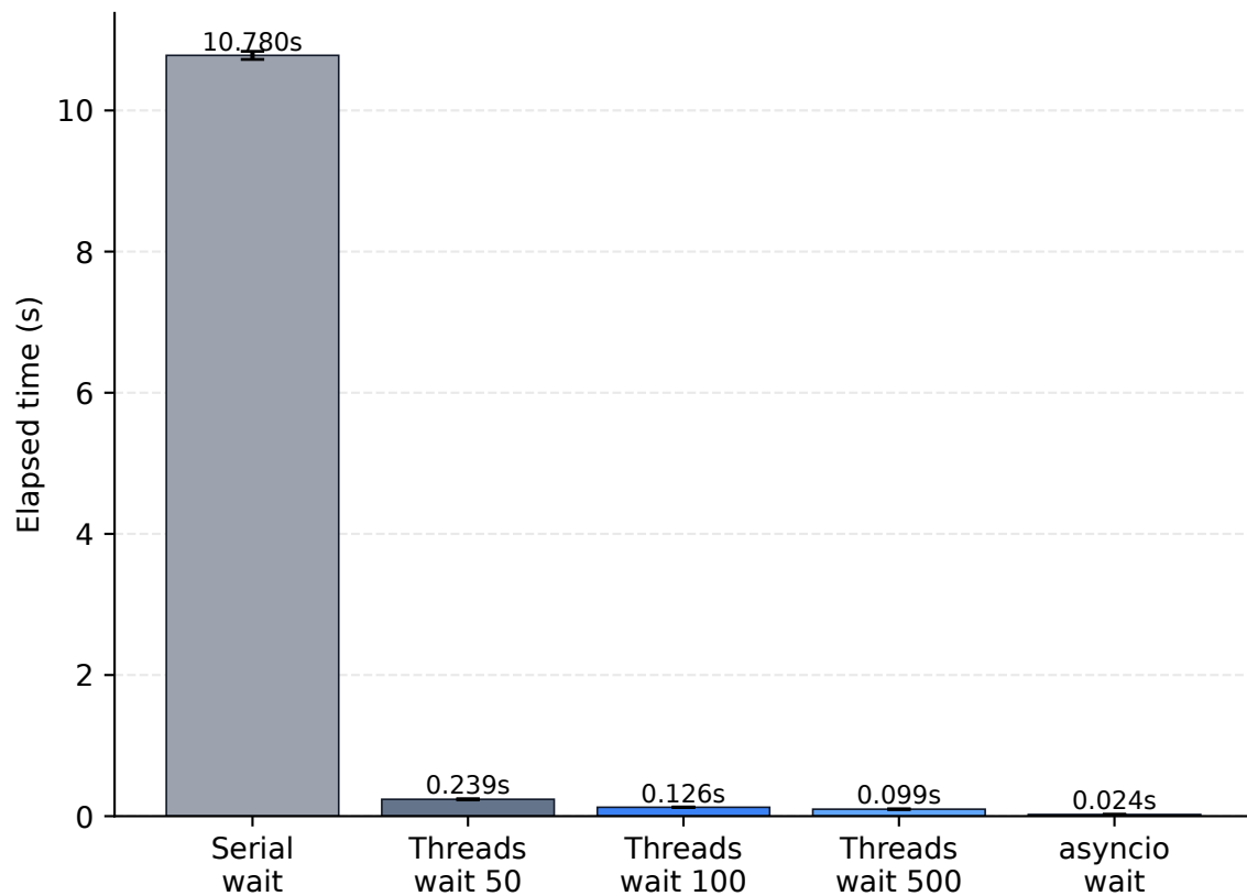
Wait-bound: 2000 tasks, 5 ms each
