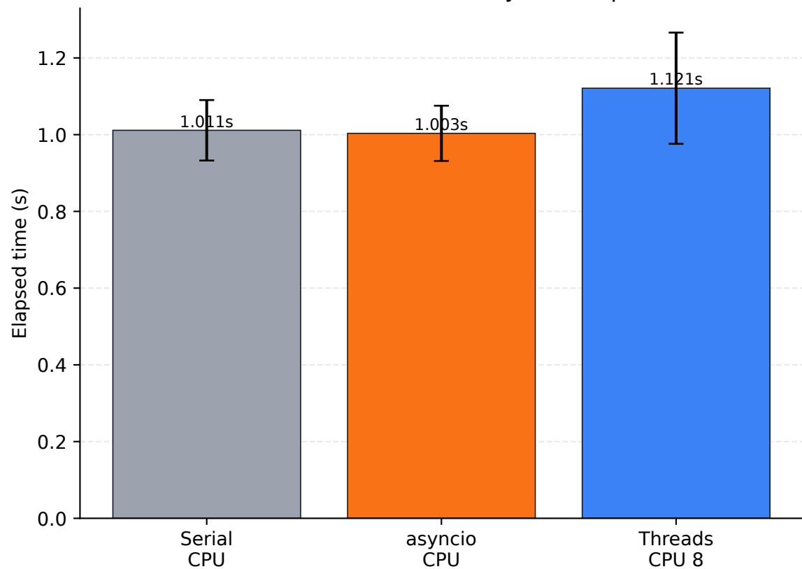
CPU-bound: 80 tasks, 120,000 Python-loop iterations
